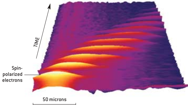
POOLS OF ELECTRONS in spin-polarized states are dragged more than 100 microns by an electric field—a fundamental step toward technology relying on large-scale quantum coherence. The peaks diminish as quantum coherence of the states is lost.
